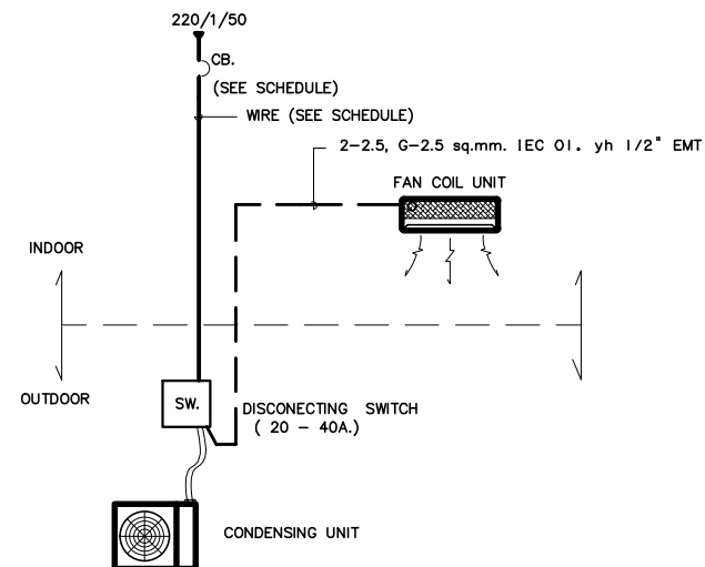
WIRING POWER SUPPLY DIAGRAM
