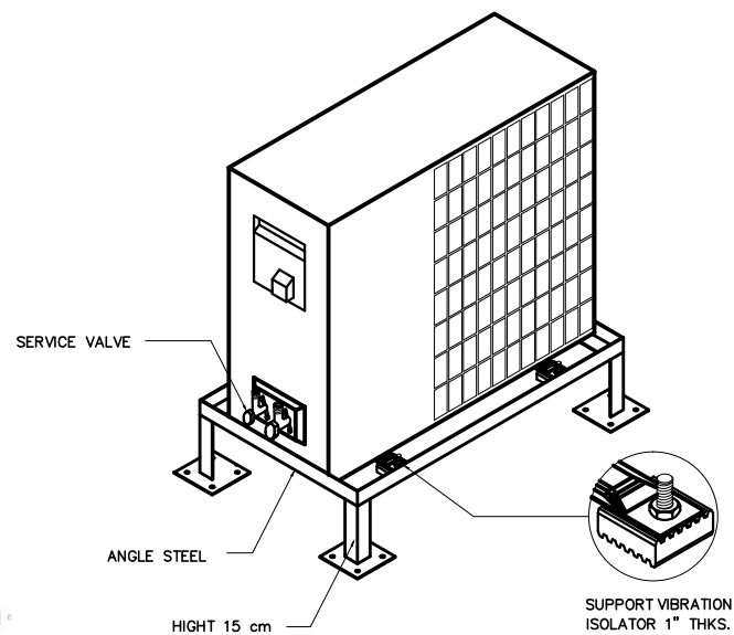
CONDENSING UNIT
